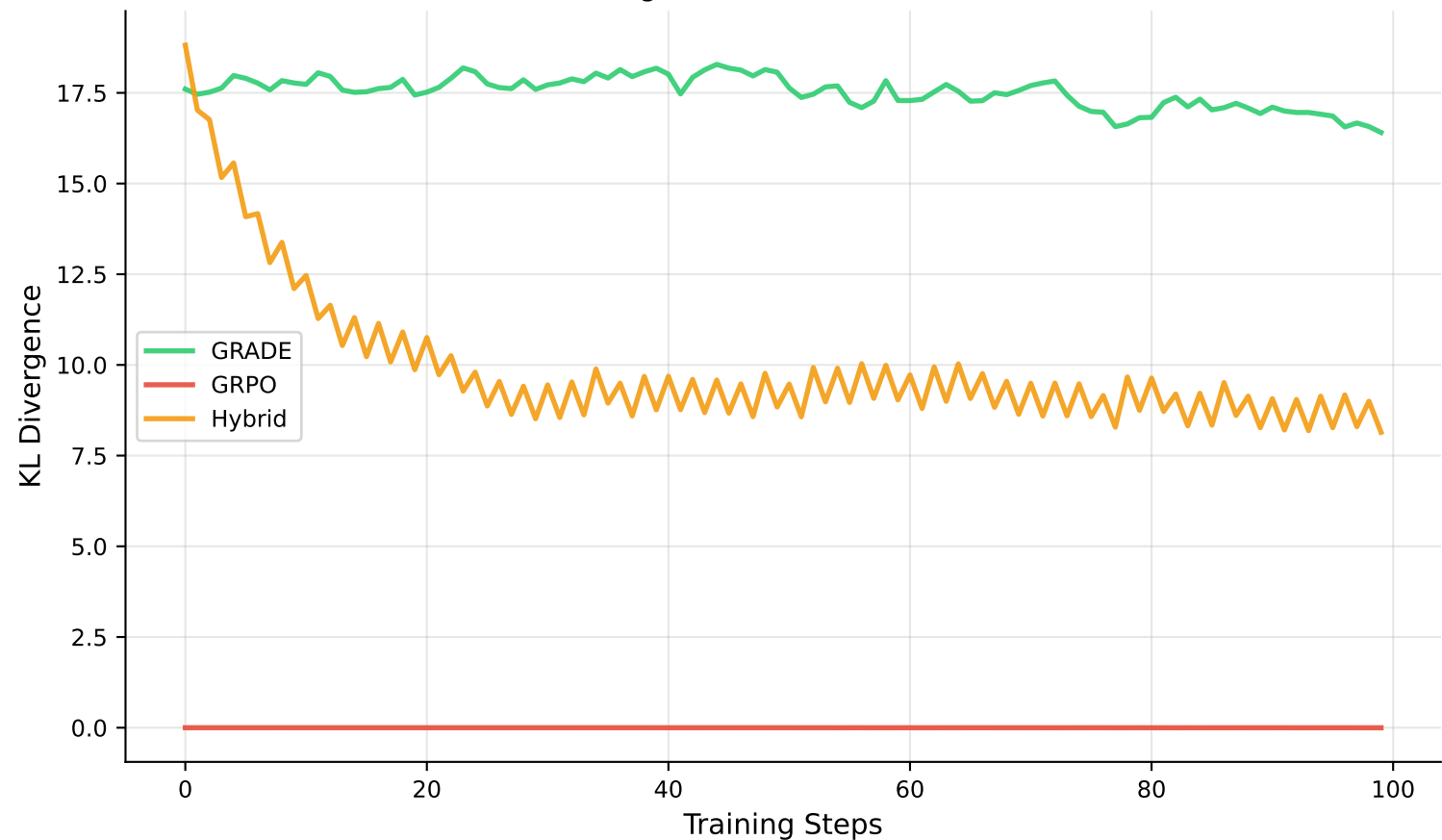
KL Divergence from Reference Model
